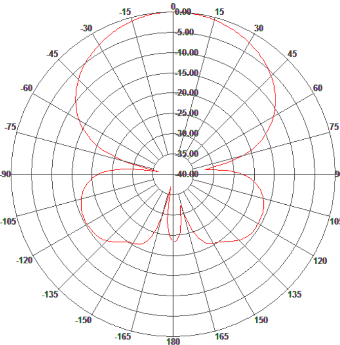
Azimuth Pattern
