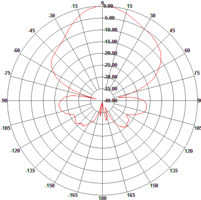
Azimuth Pattern
