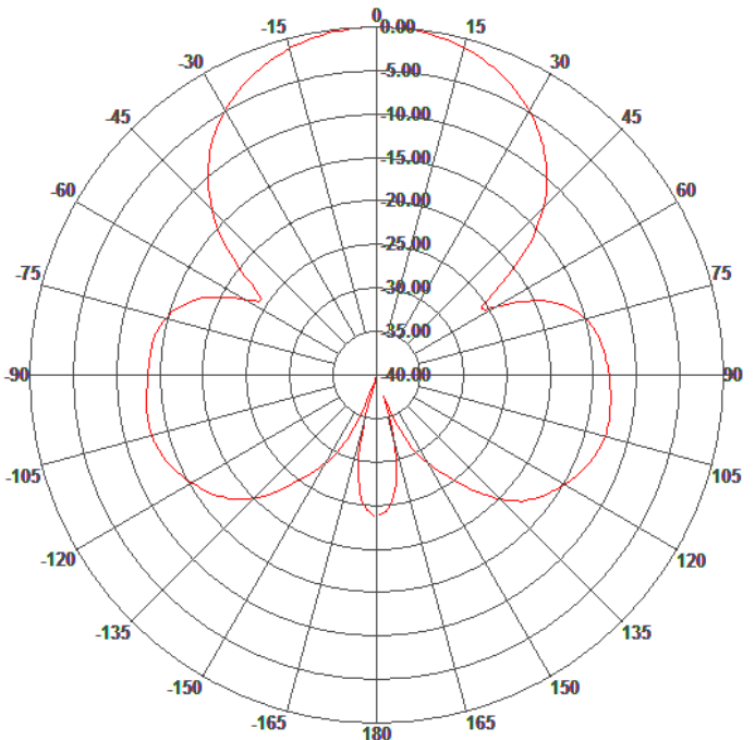
Elevation Pattern
