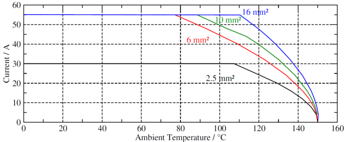
- Test according to IEC 60512-5-2, samples free in air, connected with 2.5, 6, 10 and 16mm 2 cables. Limitations possible due to different test conditions -
