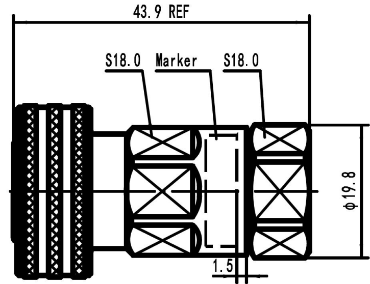
43MP-SCF12-C03 Outline drawing
