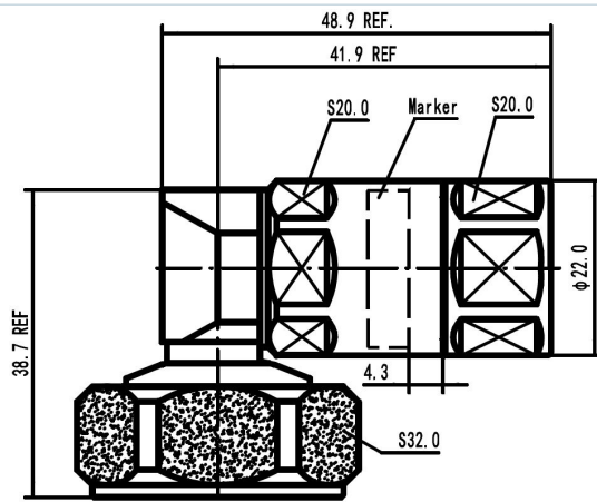
716MR-LCF12-C03 Outline drawing
