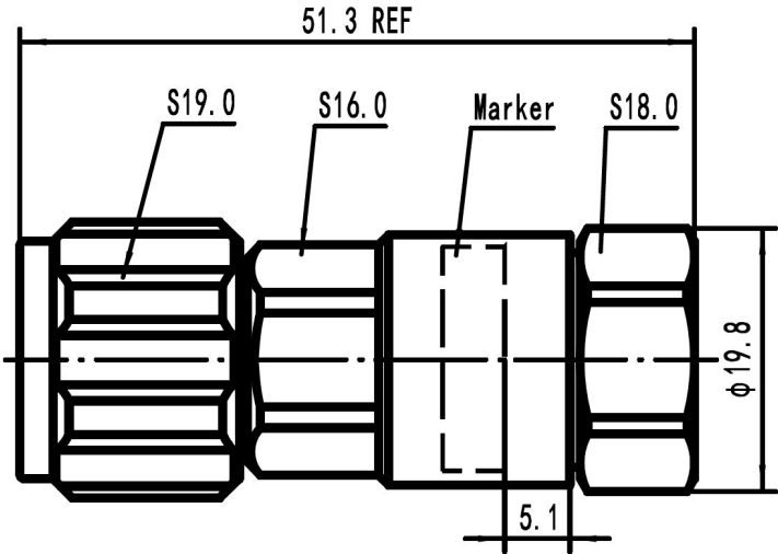
NM-SCF12-C03 Outline Drawing
