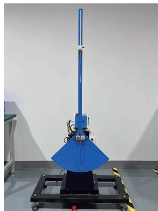
Flex Life Tester
