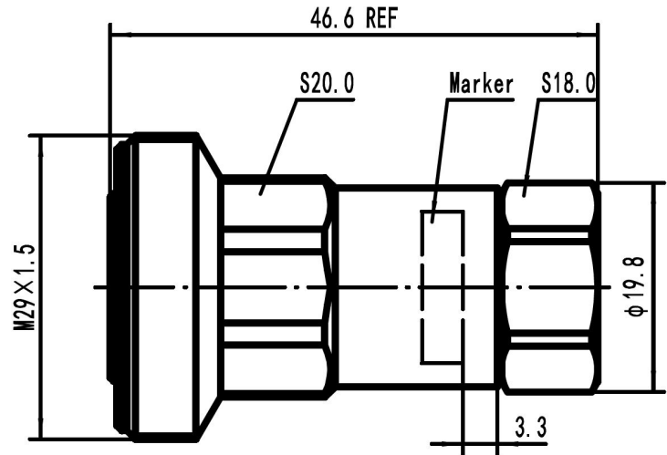
716F-SCF12-C03 Outline Drawing
